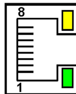
Fig. 28. View and pin numbering of the RJ45 socket
