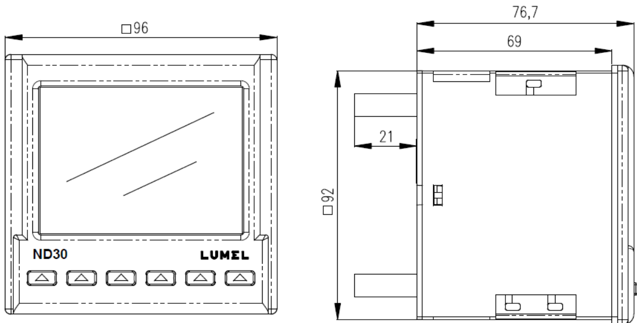
Fig. 3. Overall dimensions of the ND30 meter
